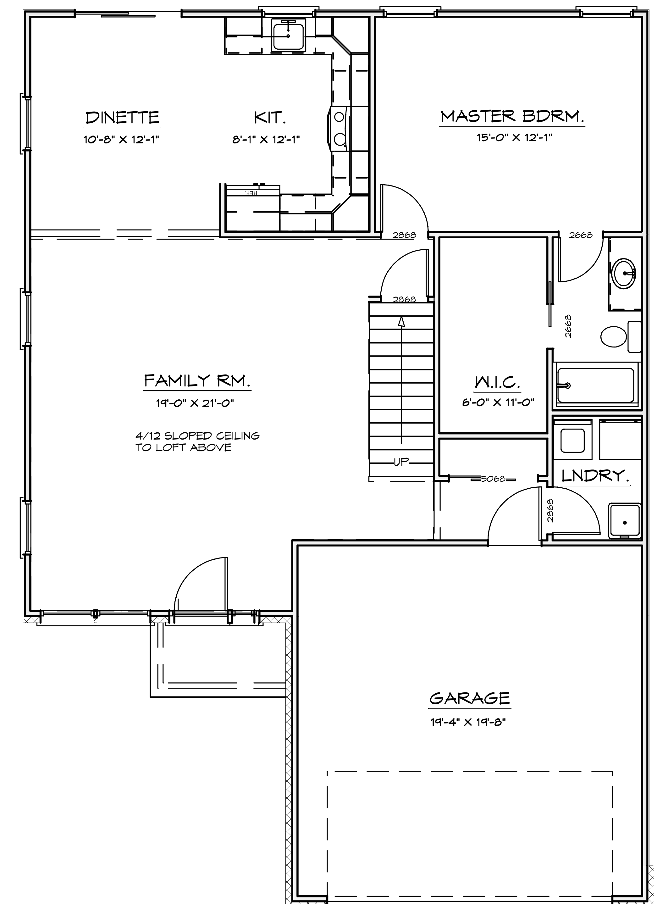
1ST FLOOR PLAN 1110 sqft
