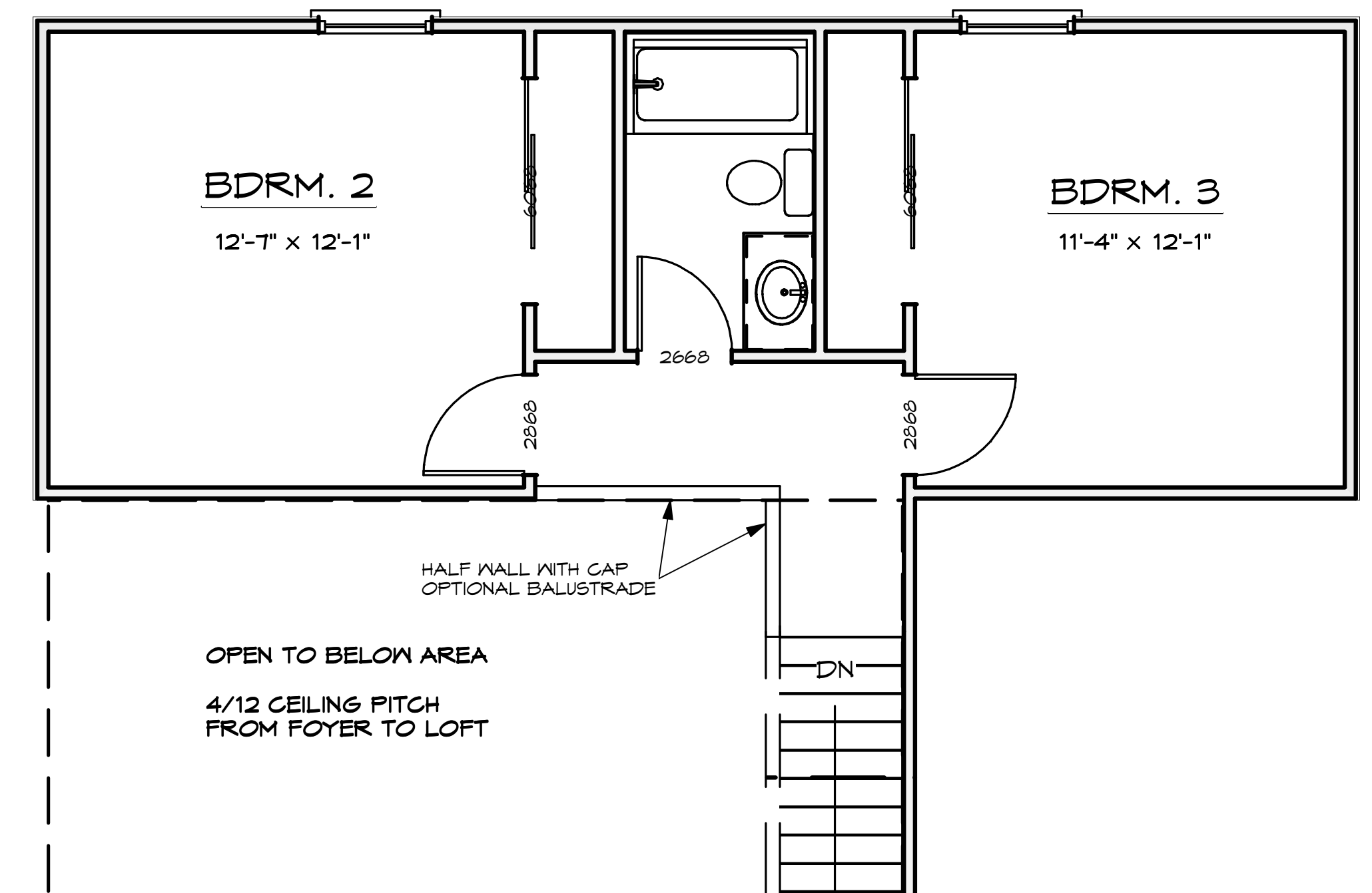
2nd FLOOR PLAN 460 sqft
